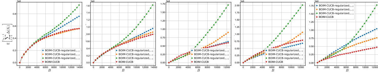
Figure 2. Regret curves on five different problem instances, with respect to the budget B (expectation computed by averaging over 10 independent simulations).
