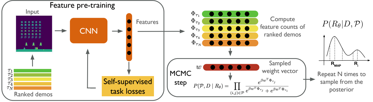
Figure 1. Bayesian Reward Extrapolation uses ranked demonstrations to pre-train a low-dimensional state feature embedding \phi(s) via self-supervised losses. After pre-training, the latent embedding function \phi(s) is frozen and the reward function is represented as a linear combination of the learned features: R(s) = w^T \phi(s) . MCMC proposal evaluations use a pairwise ranking likelihood that gives the likelihood of the preferences \mathcal{P} over demonstrations D , given a proposal w . By pre-computing the embeddings of the ranked demonstrations, \Phi_{\tau_i} , MCMC sampling is highly efficient—it does not require access to an MDP solver or data collection during inference.
