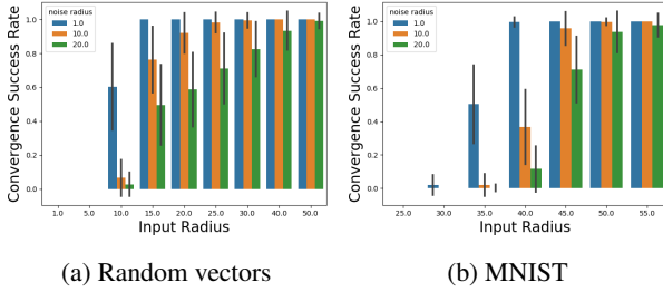
Figure 4: Convergence Success Rate vs Input Radius: 5 training examples
